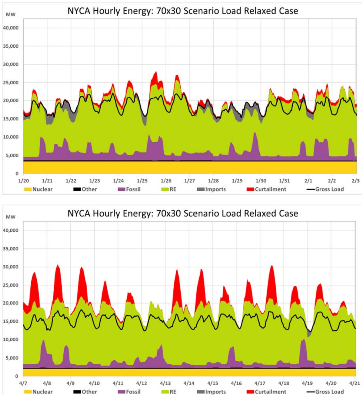
Figure 77: Sample Interval Hourly Examples: Scenario Load Relaxed Case
